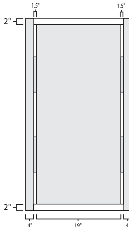
Bottom View:
