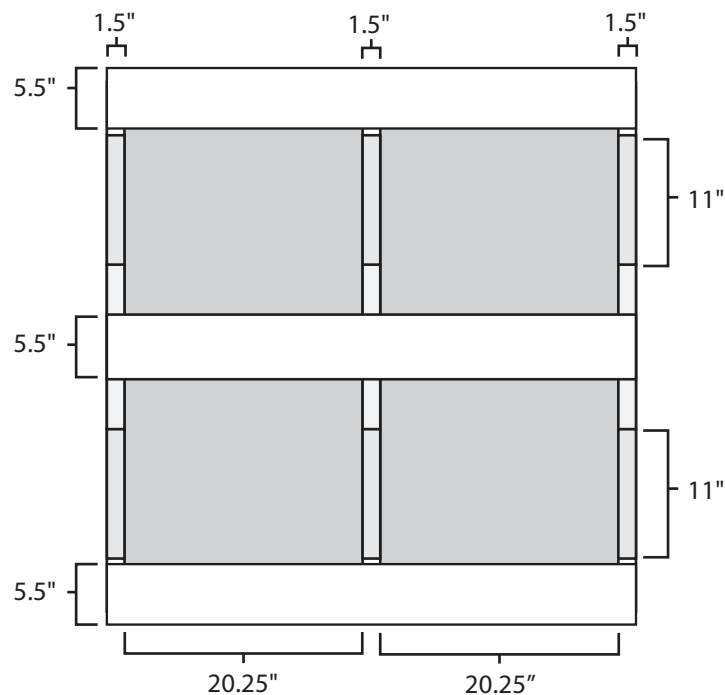
Bottom View:
