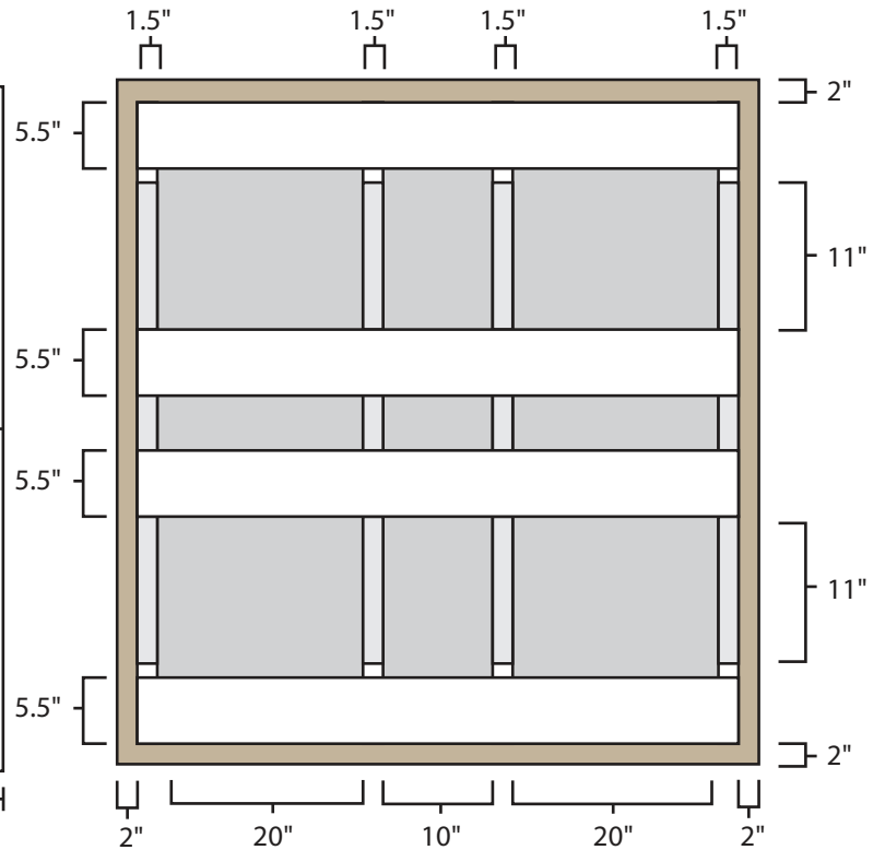
Bottom View:
