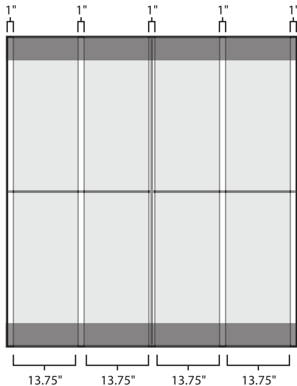
Bottom View:
